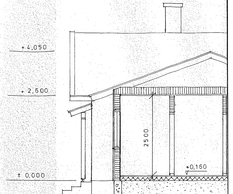
SKÄRNING A - A
